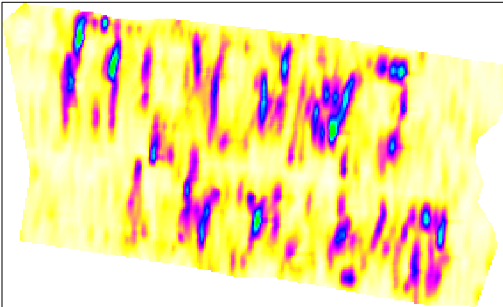
Figure 1 - Time/depth slice at 0.2m below the surface showing the individual burials. The blue and purple features are areas of high amplitude and in this case, shows the edges of the individual burial pits. The orientation of this image is the same as the site layout in Figure 3.
