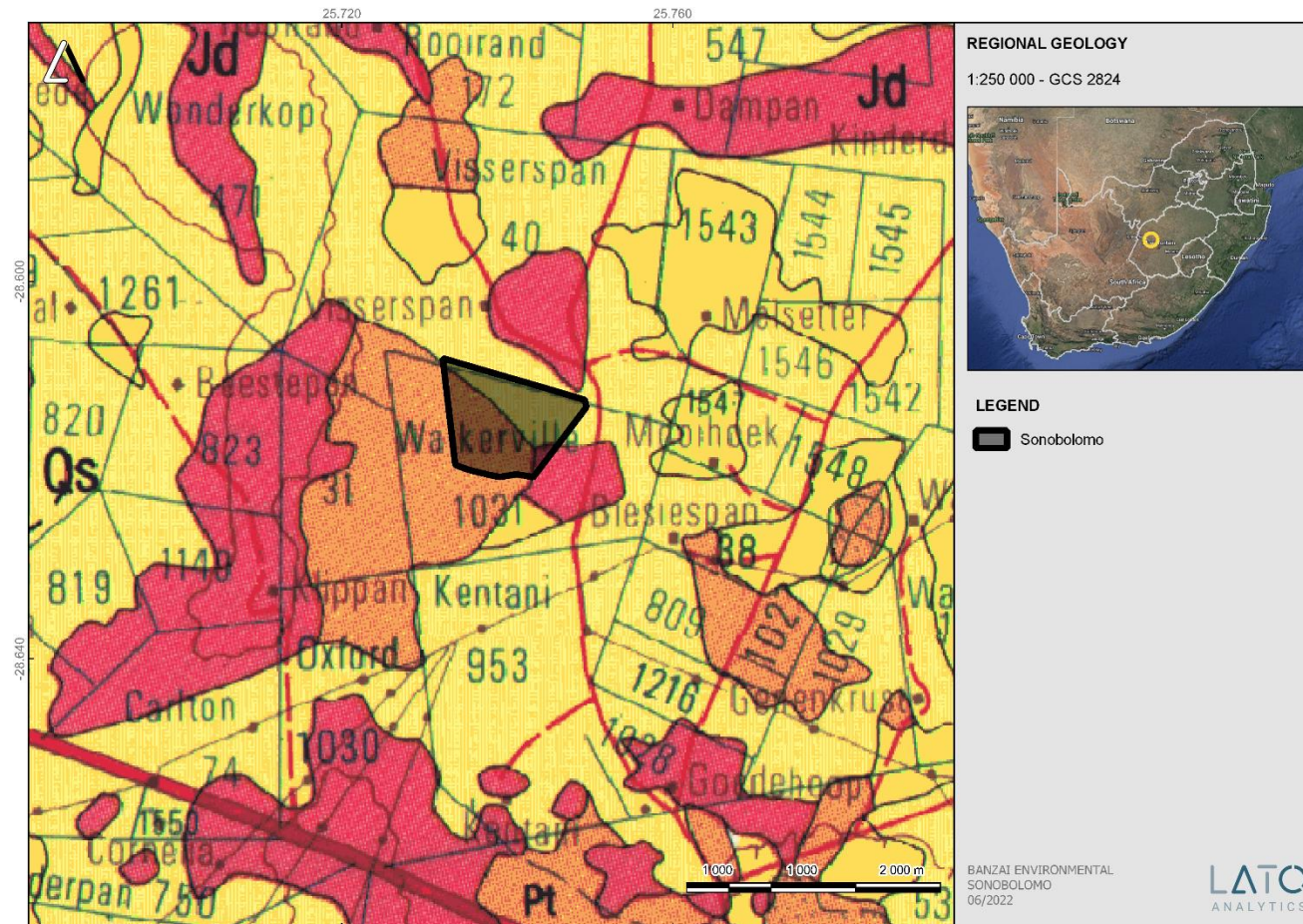
Figure 6 – Extract of the 1:250 000 Kimberley 2824 (1989) Geological map (Council of Geoscience, Pretoria) indicating the surface geology of the proposed development. The study area is underlain by Quaternary sediments (Qs; yellow) mantling the Jurassic dolerite (Jd, red), and the Tierberg Formation (Pt; orange) of the Ecca Group (Karoo Supergroup).
