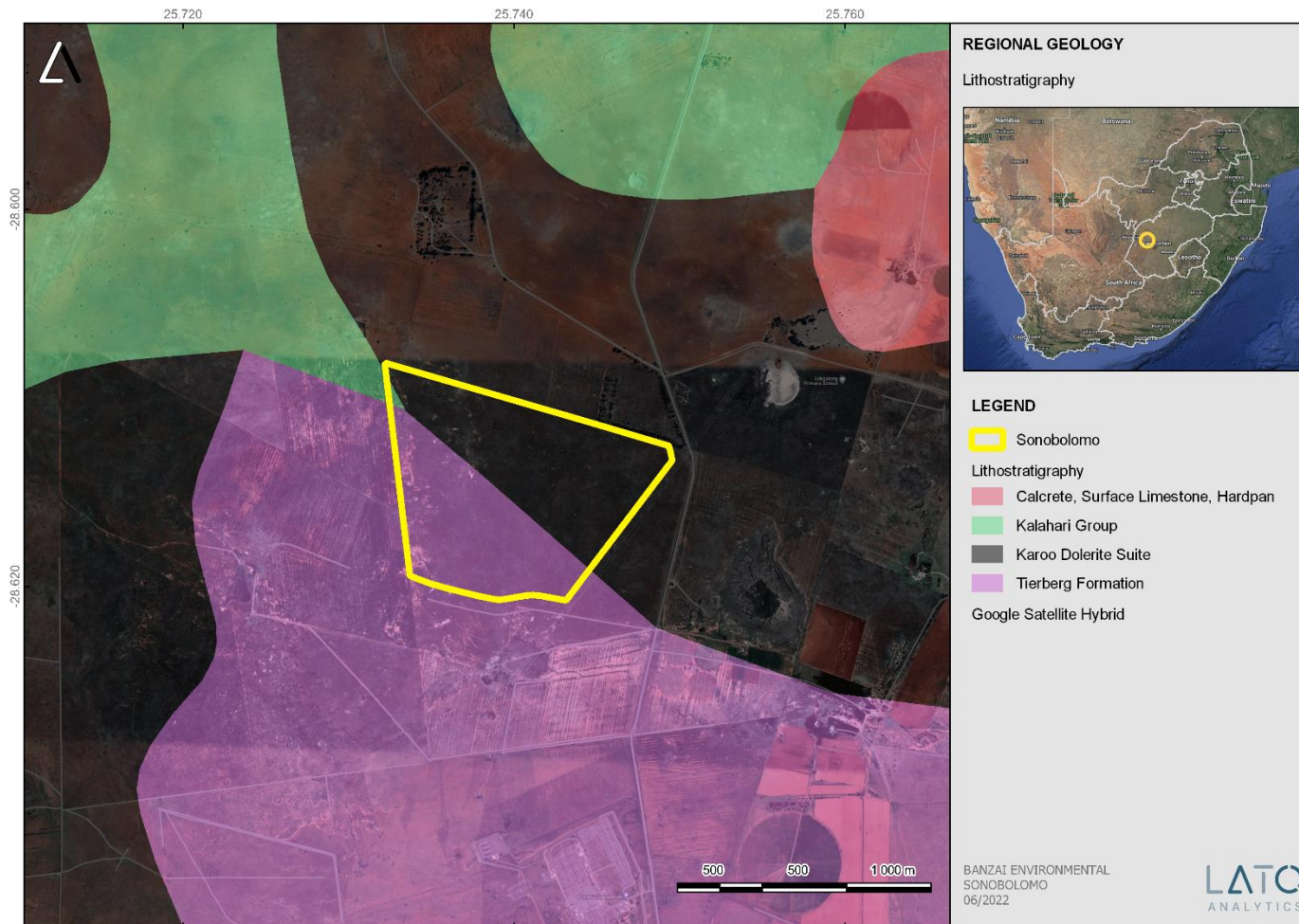
Figure 7 – Geology indicated by Shape Files (compiled by the Council of Geosciences, Pretoria). The proposed development is underlain the Karoo Dolerite as well as the Tierberg Formation.
