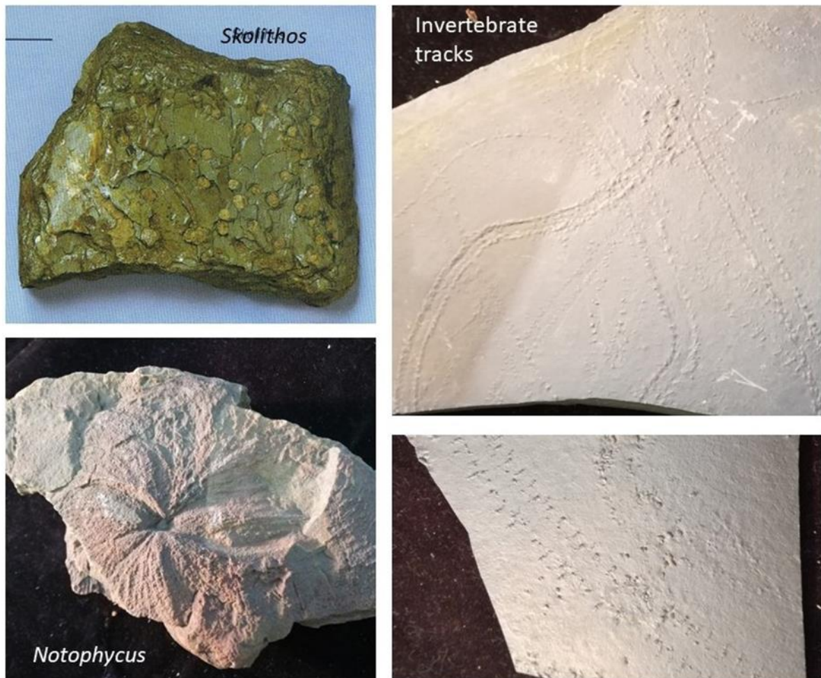
Figure 6: Photographs of trace fossils from the Ecca Group, Tierberg Formation as might be seen in the field.
