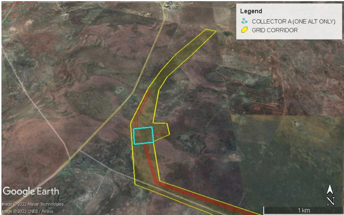
Figure 2: Google Earth Map of the proposed Collector A (turquoise square) on Remainder of Farm Corneliasdal No. 45 in the western side of the Dealesville Springhaas Solar PV Facility.
