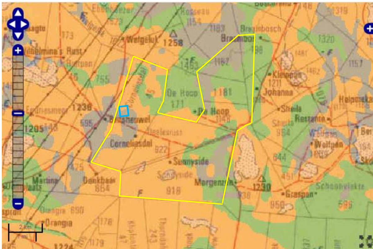
Figure 4: SAHRIS Palaeosensitivity map for the site for the proposed Collector substation A (approximate location), blue box. Broader study area, yellow Background colours indicate the following degrees of sensitivity: red = very highly sensitive; orange/yellow = high; green = moderate; blue = low; grey = insignificant/zero.
