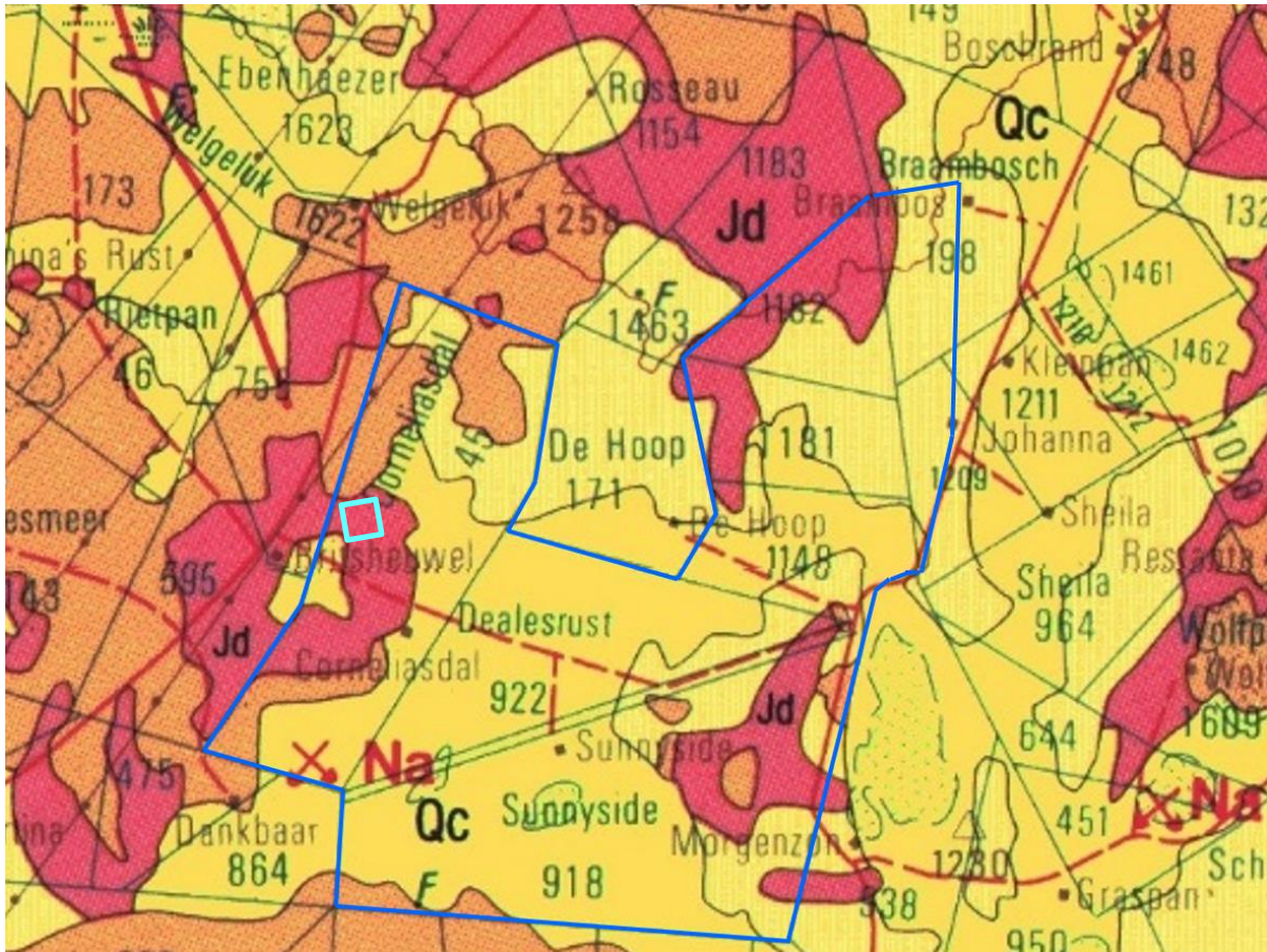
Figure 3: Geological map of the area around the Dealesville Springhaas Solar PV Facility (blue outline). Small turquoise square (west) indicates the approximate location of Collector A. Abbreviations of the rock types are explained in Table 2. Map enlarged from the Geological Survey 1: 250 000 map 2824 Kimberley.
