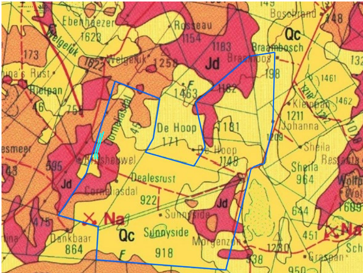
Figure 3: Geological map of the area around the Dealesville Springhaas Solar PV Facility (blue outline). Turquoise line indicates the approximate location of LiLo 1. Abbreviations of the rock types are explained in Table 2. Map enlarged from the Geological Survey 1: 250 000 map 2824 Kimberley.
