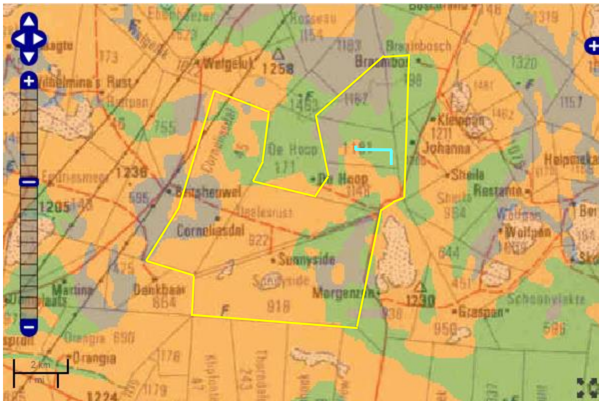
Figure 4: SAHRIS Palaeosensitivity map for the site for the proposed Line 1, turquoise line. Broader study area, yellow Background colours indicate the following degrees of sensitivity: red = very highly sensitive; orange/yellow = high; green = moderate; blue = low; grey = insignificant/zero.
