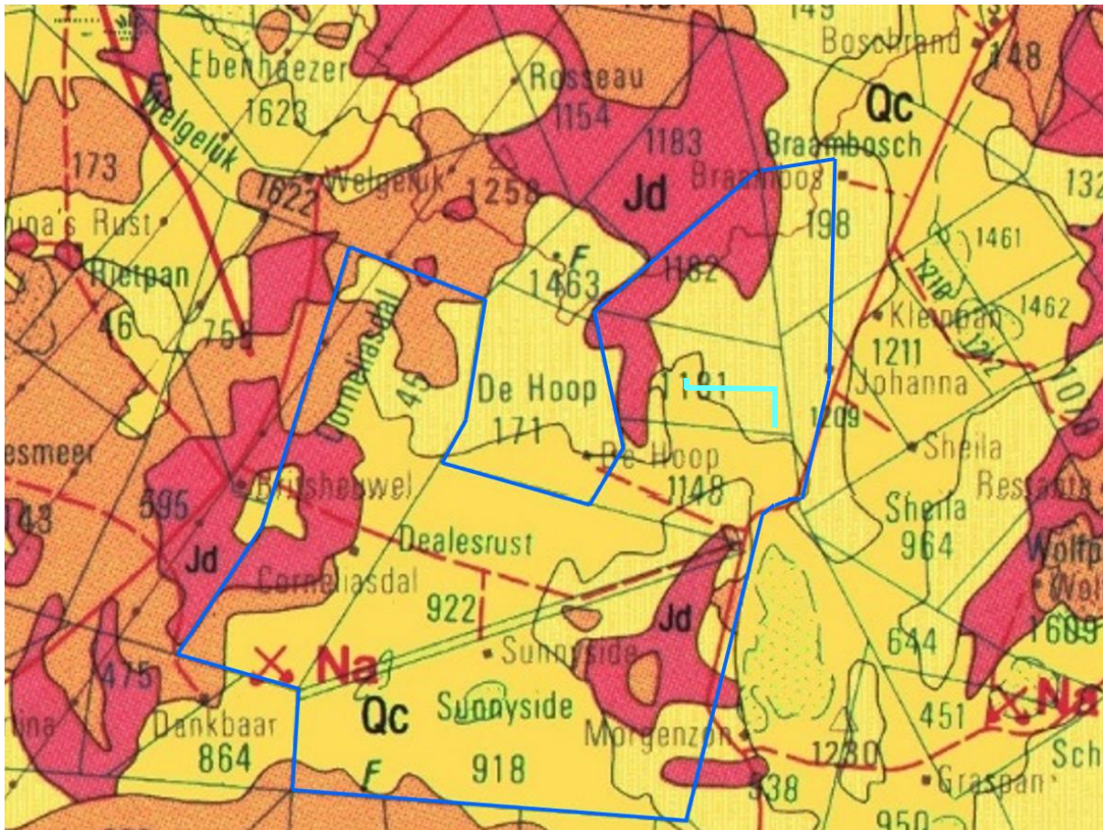
Figure 3: Geological map of the area around the Dealesville Springhaas Solar PV Facility (blue outline). t Turquoise line indicates the approximate location of Line 1. Abbreviations of the rock types are explained in Table 2. Map enlarged from the Geological Survey 1: 250 000 map 2824 Kimberley.
