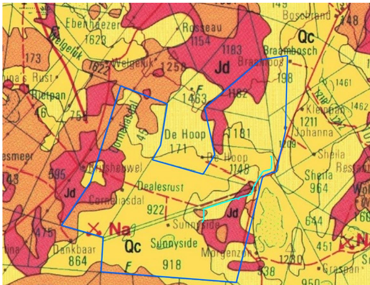
Figure 3: Geological map of the area around the Dealesville Springhaas study area (blue outline). Turquoise line indicates the approximate location of Line 5. Abbreviations of the rock types are explained in Table 2. Map enlarged from the Geological Survey 1: 250 000 map 2824 Kimberley.
