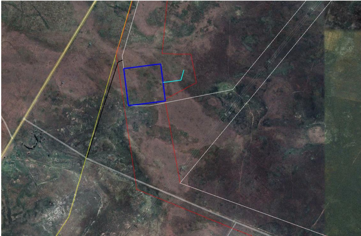
Figure 2: Google Earth Map of the proposed Line 6 (turquoise line) on Remainder of Farm Corneliasdal No. 45, also shown in the figure, grid corridor (red), Collector Substation A (blue), access roads (black), solar PV facility boundary (light grey), broader study area (yellow)
