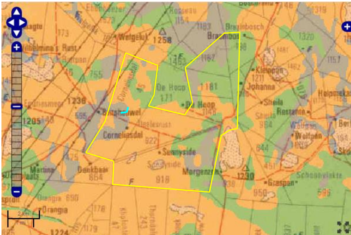
Figure 4: SAHRIS Palaeosensitivity map for the site for the proposed Line 6, turquoise line. Broader study area, yellow. Background colours indicate the following degrees of sensitivity: red = very highly sensitive; orange/yellow = high; green = moderate; blue = low; grey = insignificant/zero.
