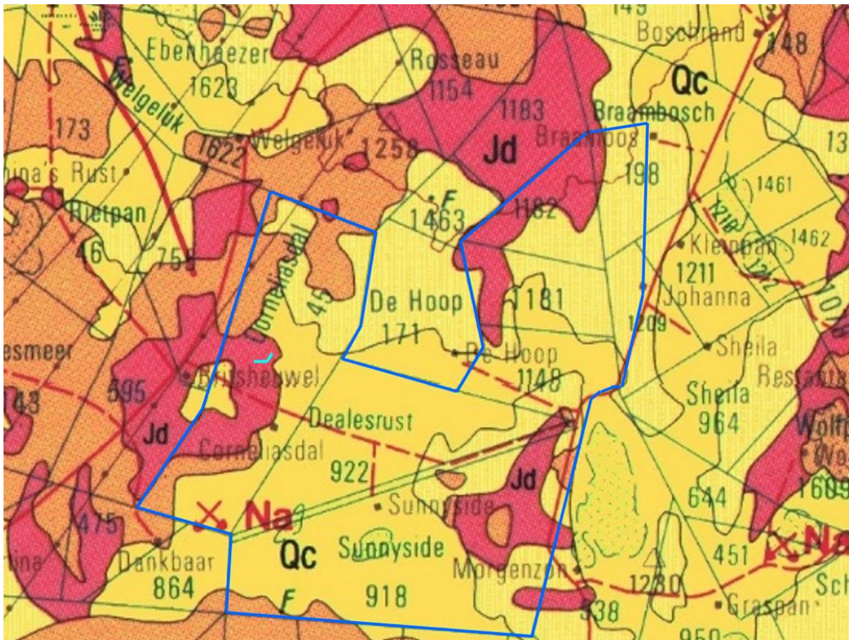
Figure 3: Geological map of the area around the Dealesville Springhaas study area (blue outline). Turquoise line indicates the approximate location of Line 6, Abbreviations of the rock types are explained in Table 2. Map enlarged from the Geological Survey 1: 250 000 map 2824 Kimberley.
