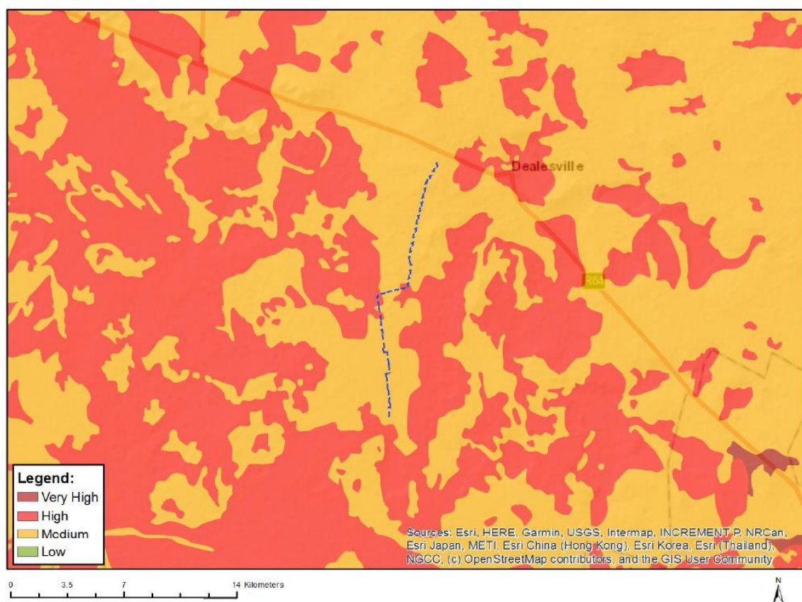
Figure 5: Map of palaeontology sensitivity for Line 2 from Springhaas Collector Substation B to the Artemis Substation
