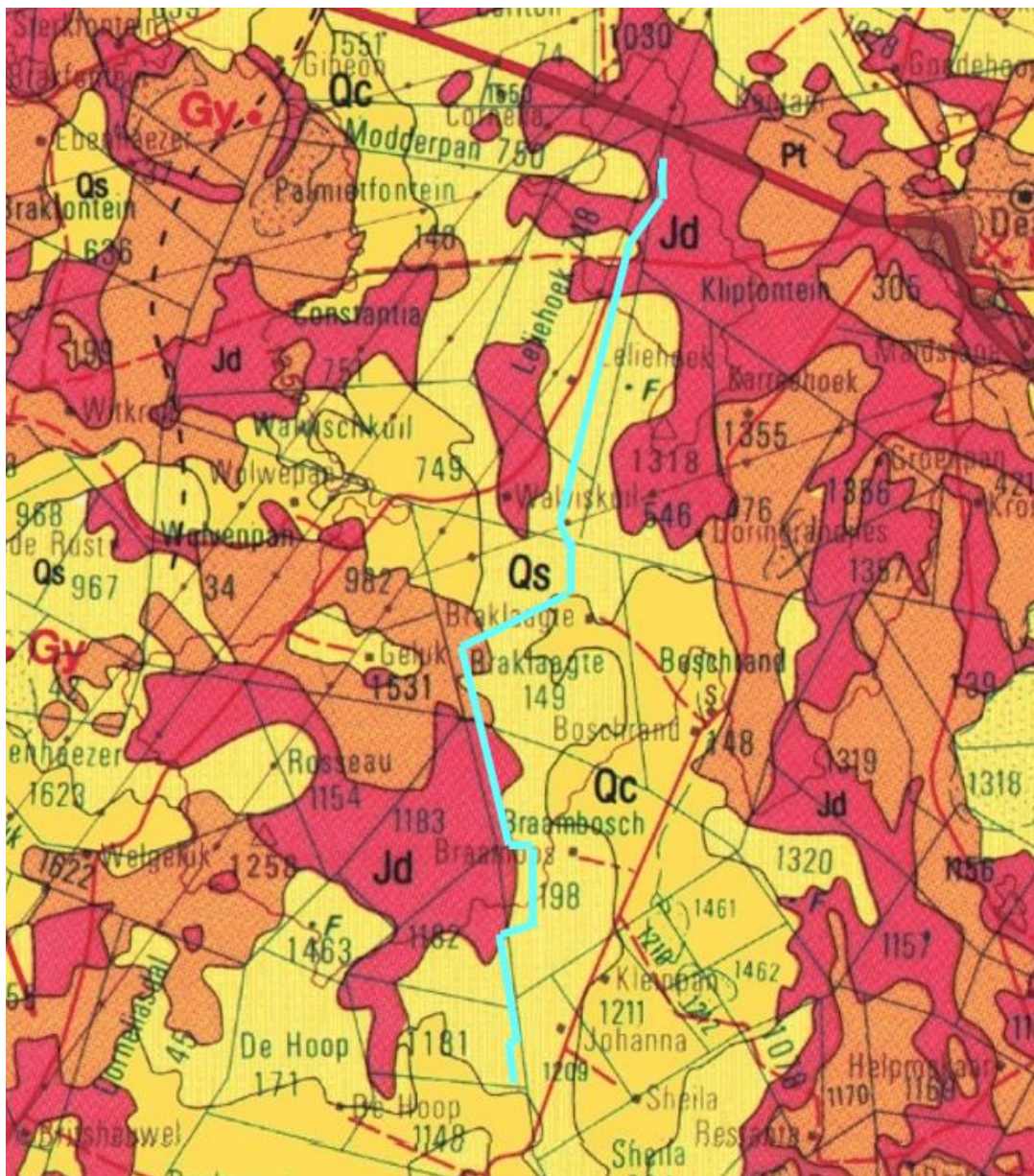
Figure 3: Geological map of the area around the Dealesville Springhaas study area. Turquoise line indicates the approximate route of Line 2. Abbreviations of the rock types are explained in Table 2. Map enlarged from the Geological Survey 1: 250 000 map 2824 Kimberley.
