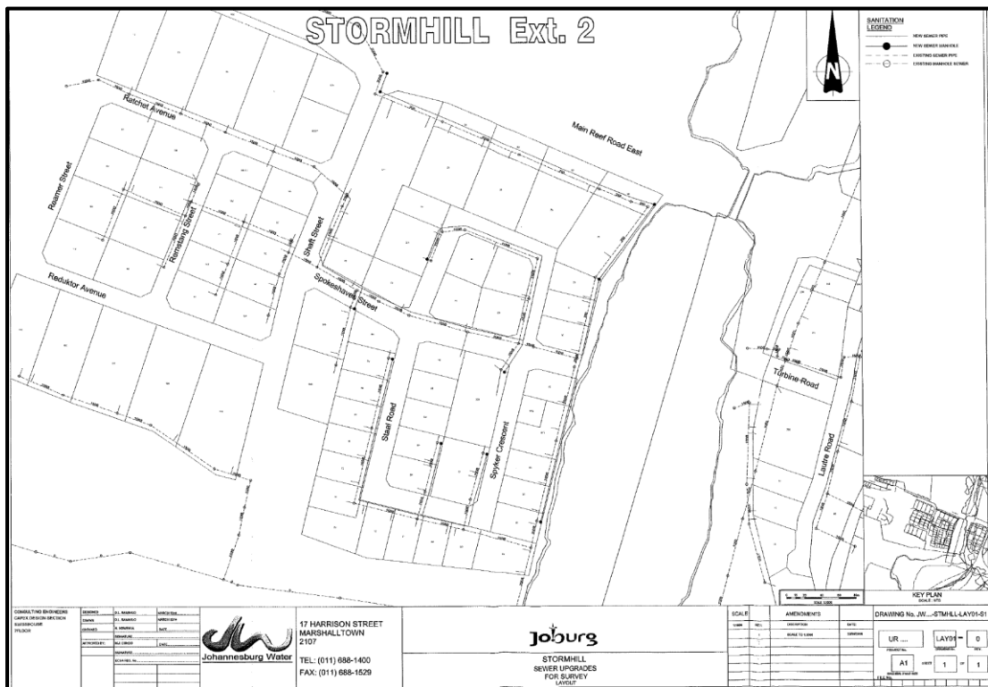
Figure 2. Layout of the proposed development
