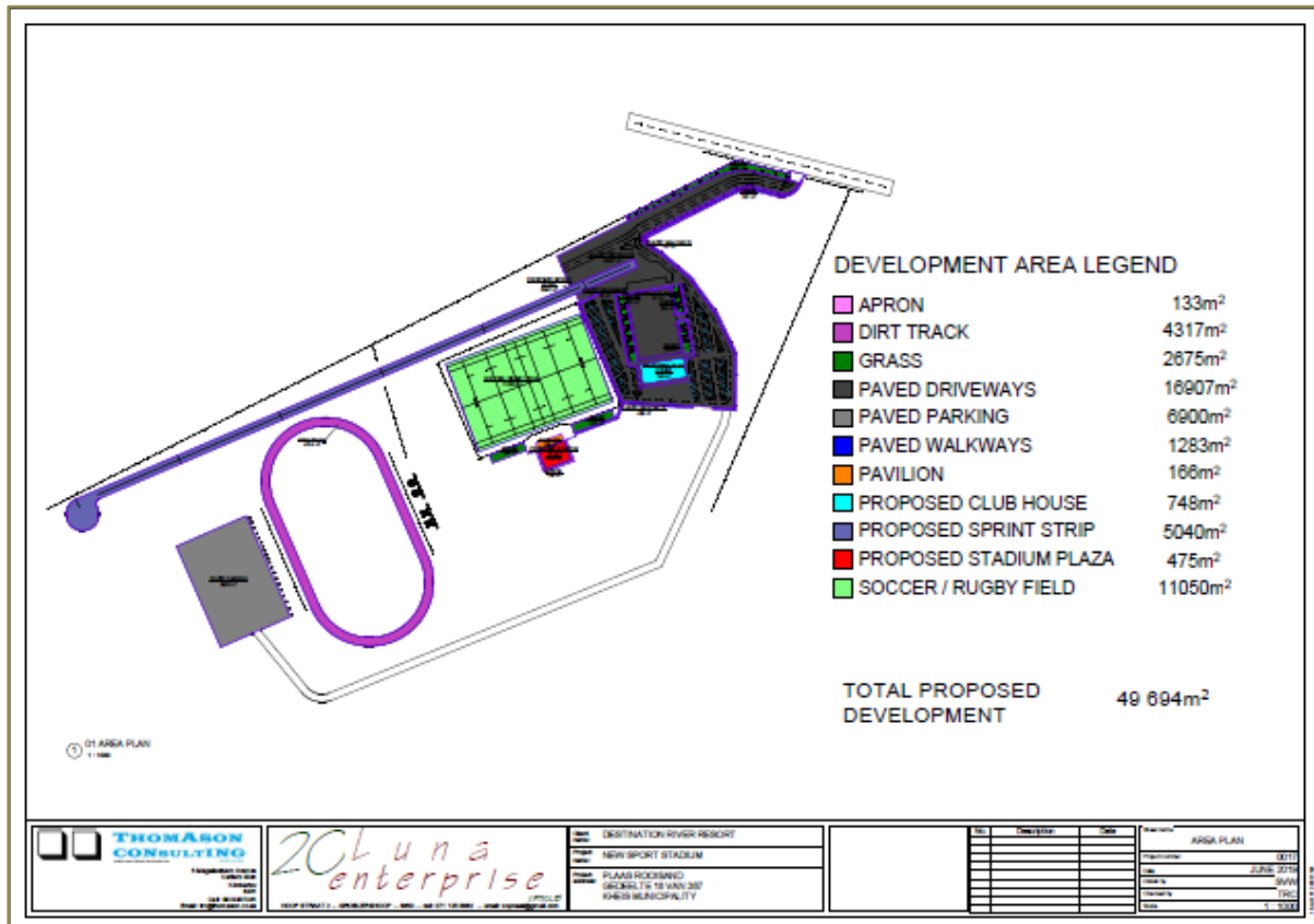
Figure 6 Sports Complex plan (provided by EnviroAfrica cc).
