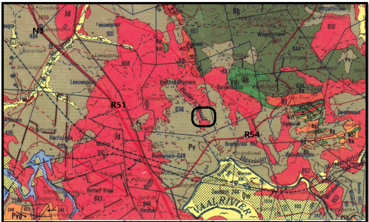
Figure 3: Excerpt of 1:250 000 Geological Map East Rand (Keyser et al. 1986) (1h).
