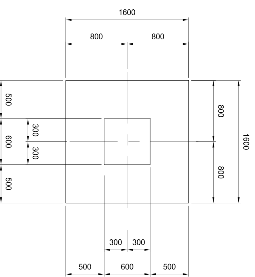
PLAN ON FOUNDATION SCALE 1 : 30
