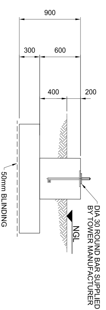
TYPICAL SECTION SCALE 1 : 30
