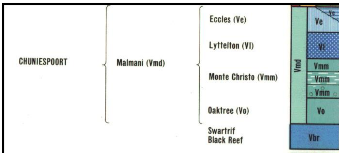
Figure 6: Lithostratigraphy (Keyser 1986).
