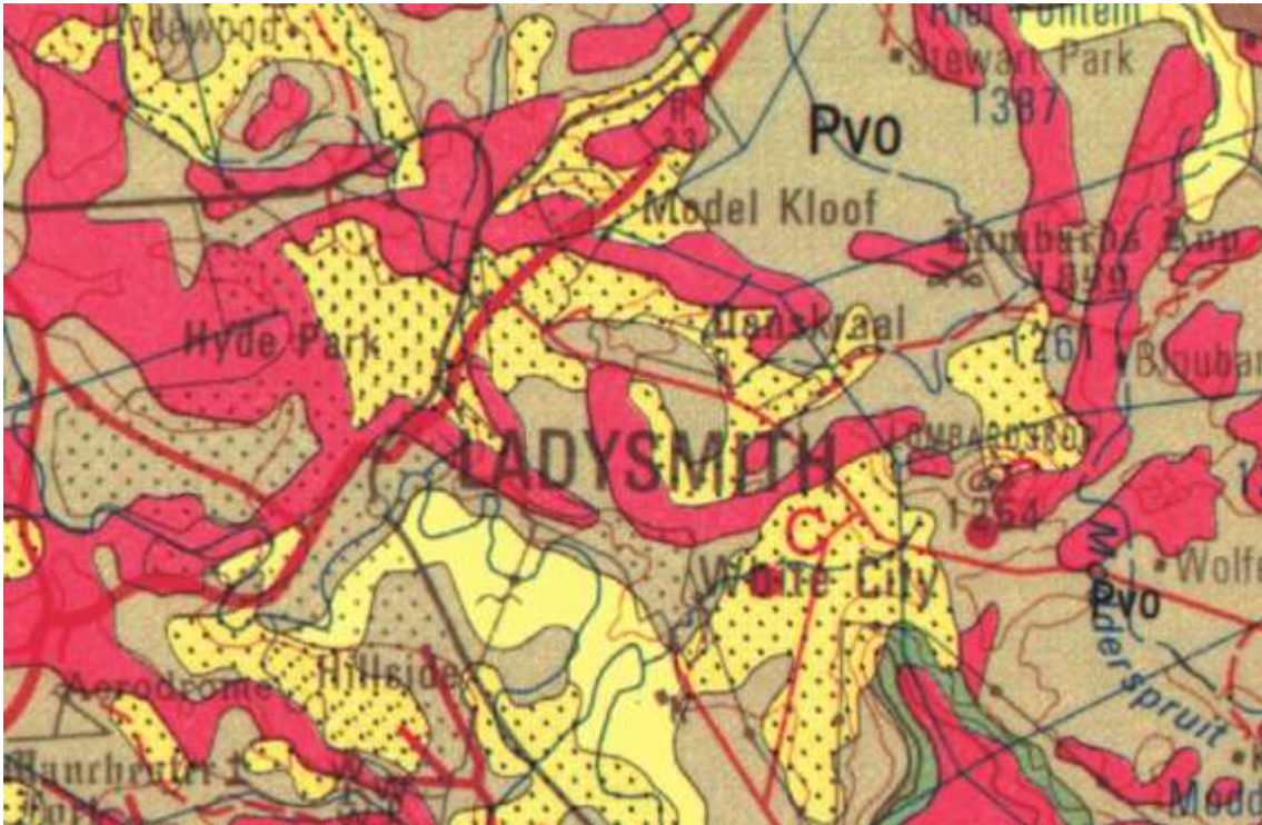
Figure 2 (a): Extract from the Harrismith (2828) 1: 250 000 Geological Map. Grey (Pvo) is the Volksrust Formation, red is Karoo Dolerite and the yellow is Quaternary sediments.
